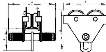
Plain trolley
