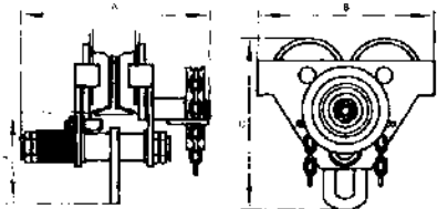
Geared trolley
